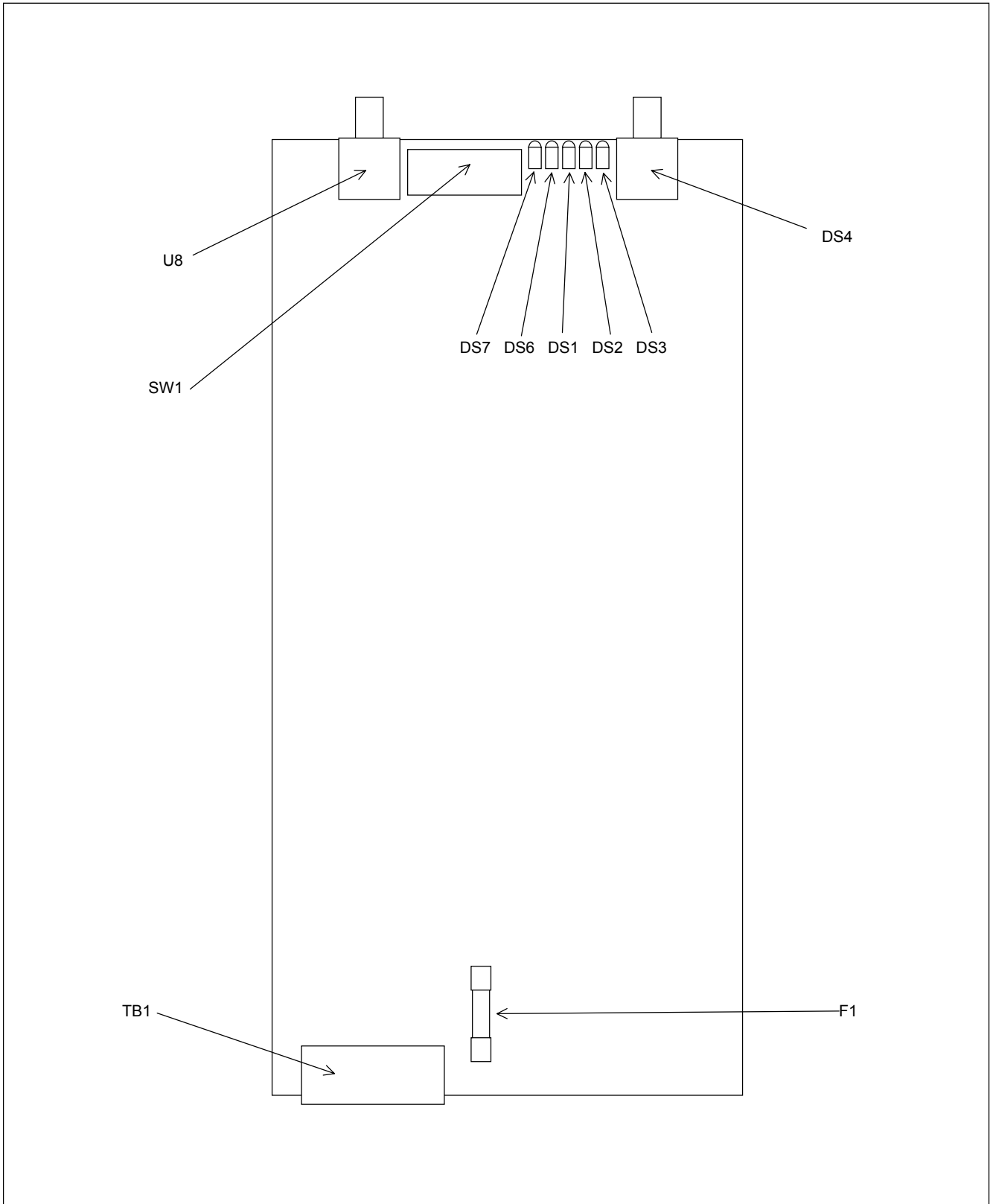
Figure 8. Fiber Service Unit ECB No. 107463-5 (Board A), controls and indicators (107460-5)
