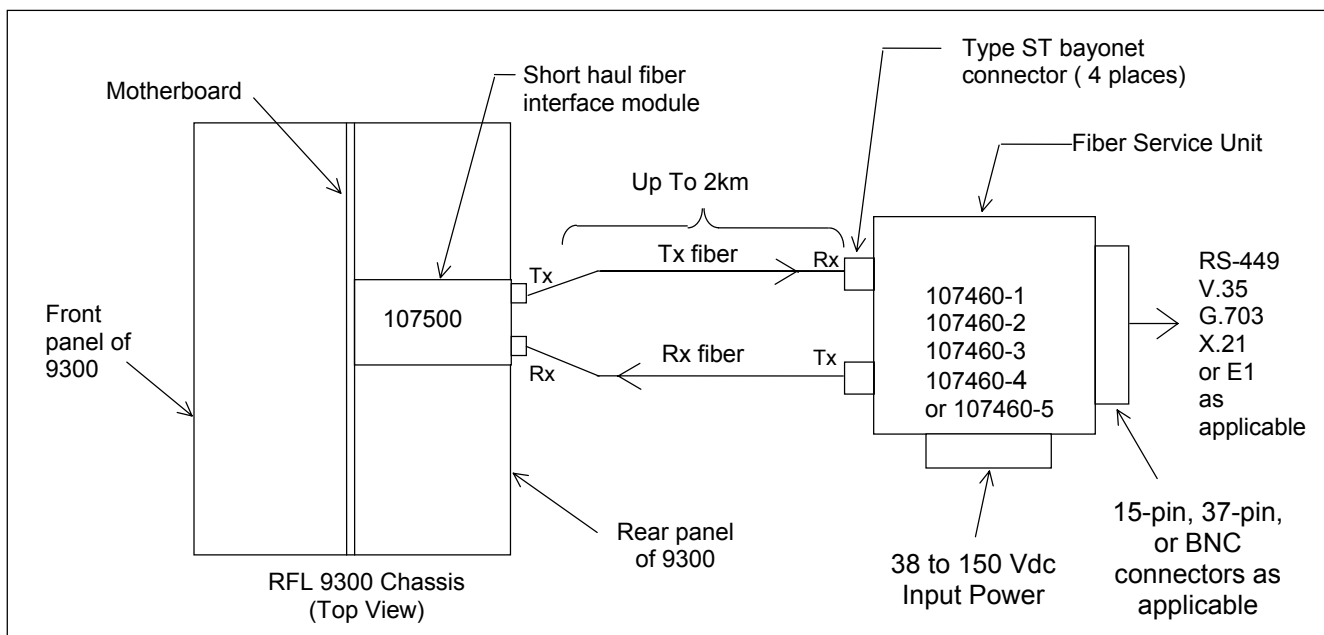
Figure 2. Connecting the FSU to an RFL 9300
