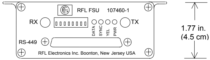
a. Fiber Service Unit front view
