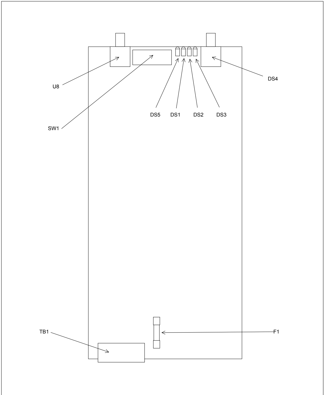
Figure 6. Fiber Service Unit ECB No. 107463 (Board A), controls and indicators (107460-1 to 107460-4)
