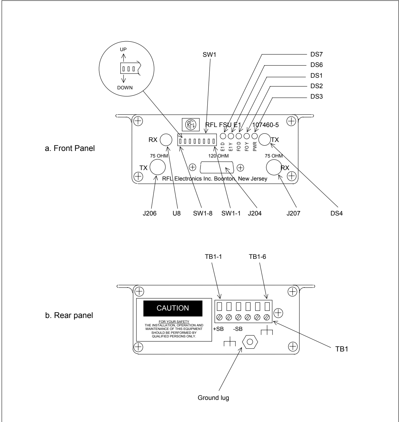
Figure 7. Fiber Service Unit, front and rear panel controls and indicators (107460-5)
