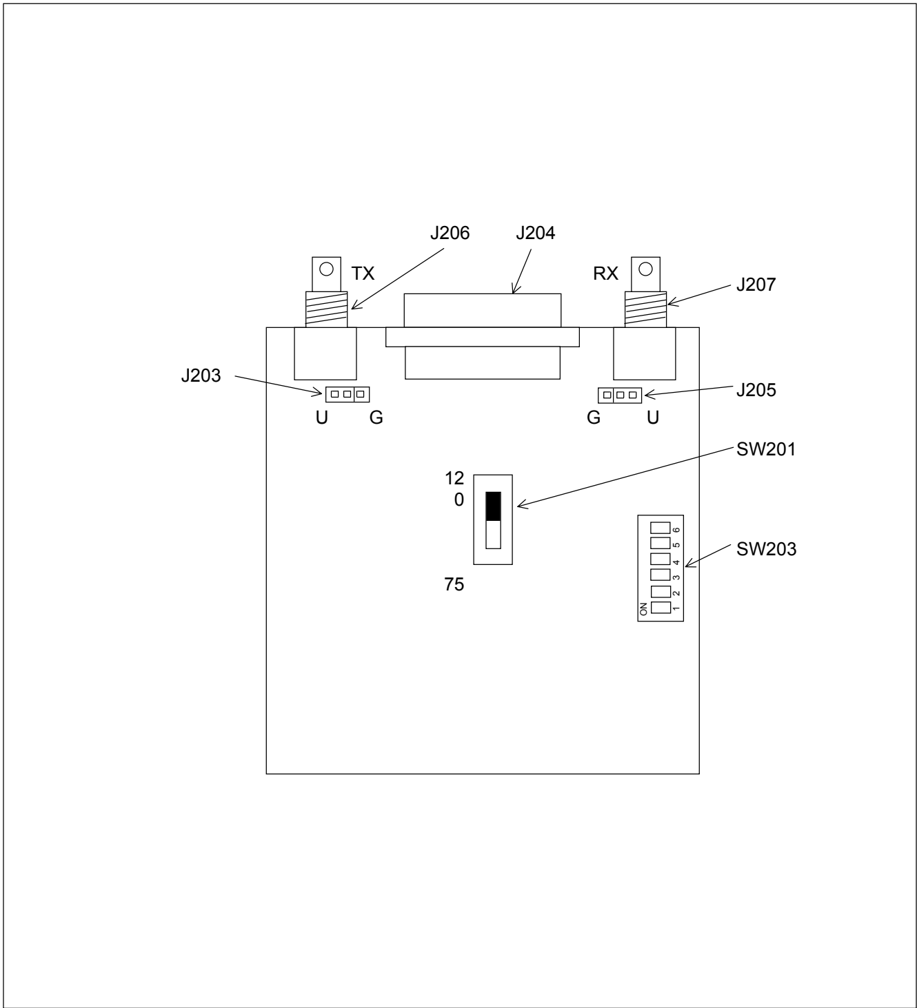
Figure 9. Fiber Service Unit ECB No. 107463-5 Board B
