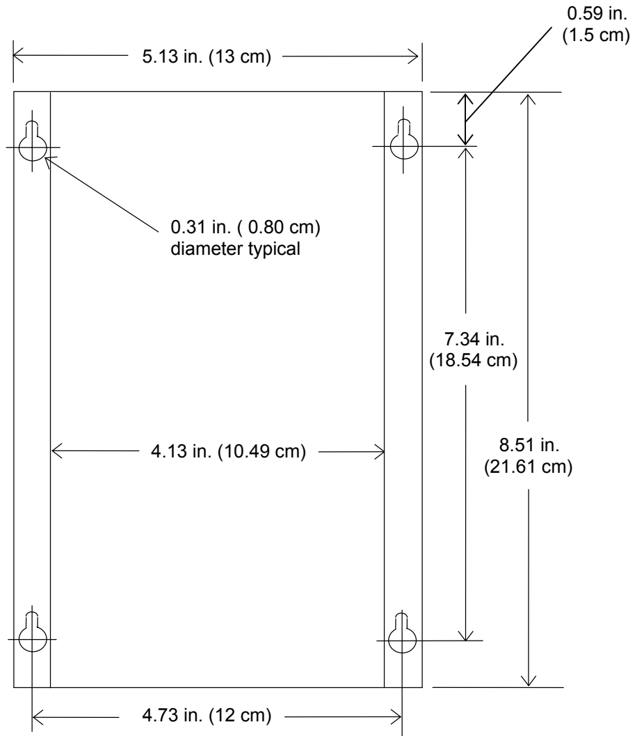
b. Fiber Service Unit top view
