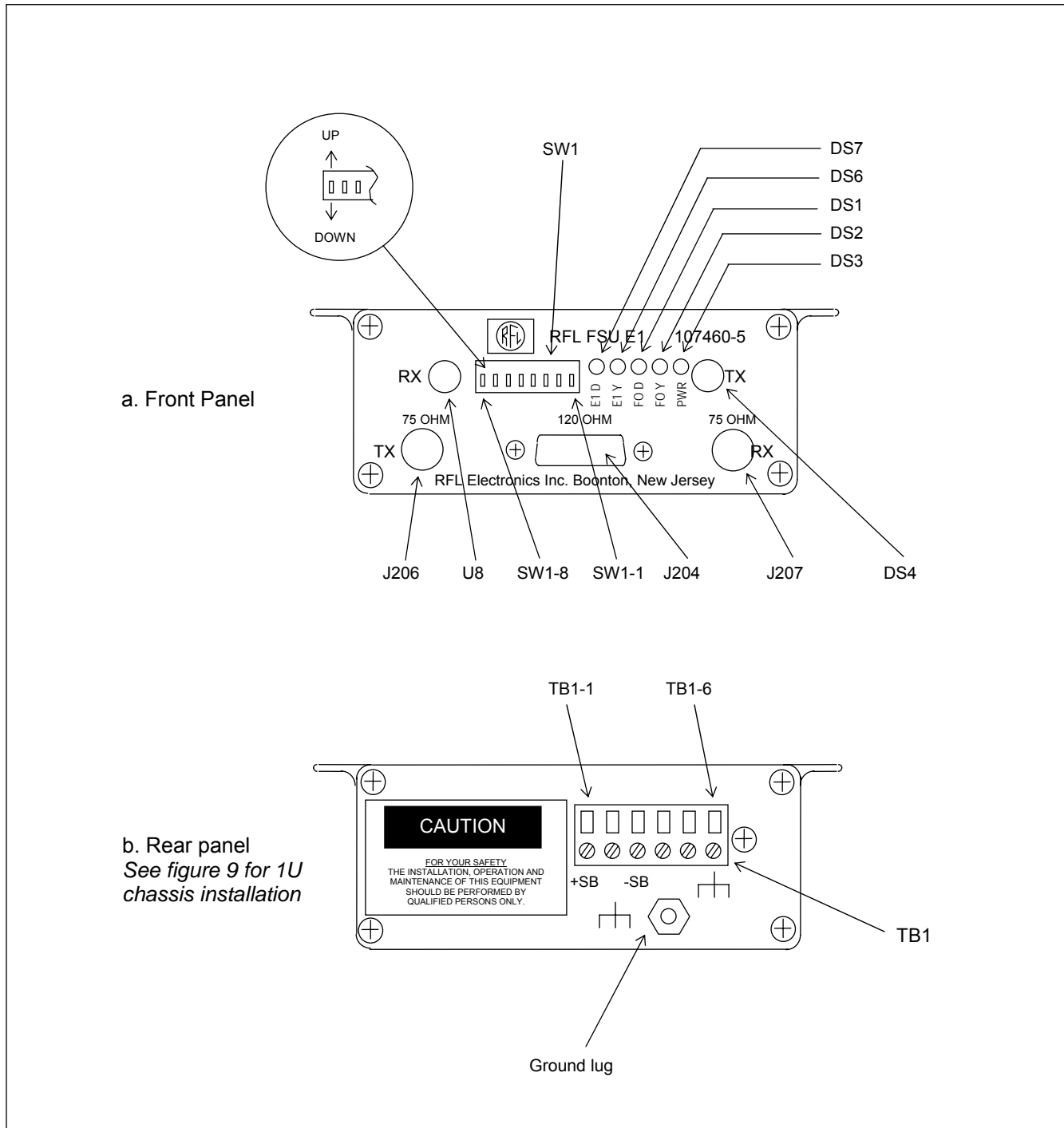
Figure 8. Fiber Service Unit, front and rear panel controls and indicators (107460-5)
