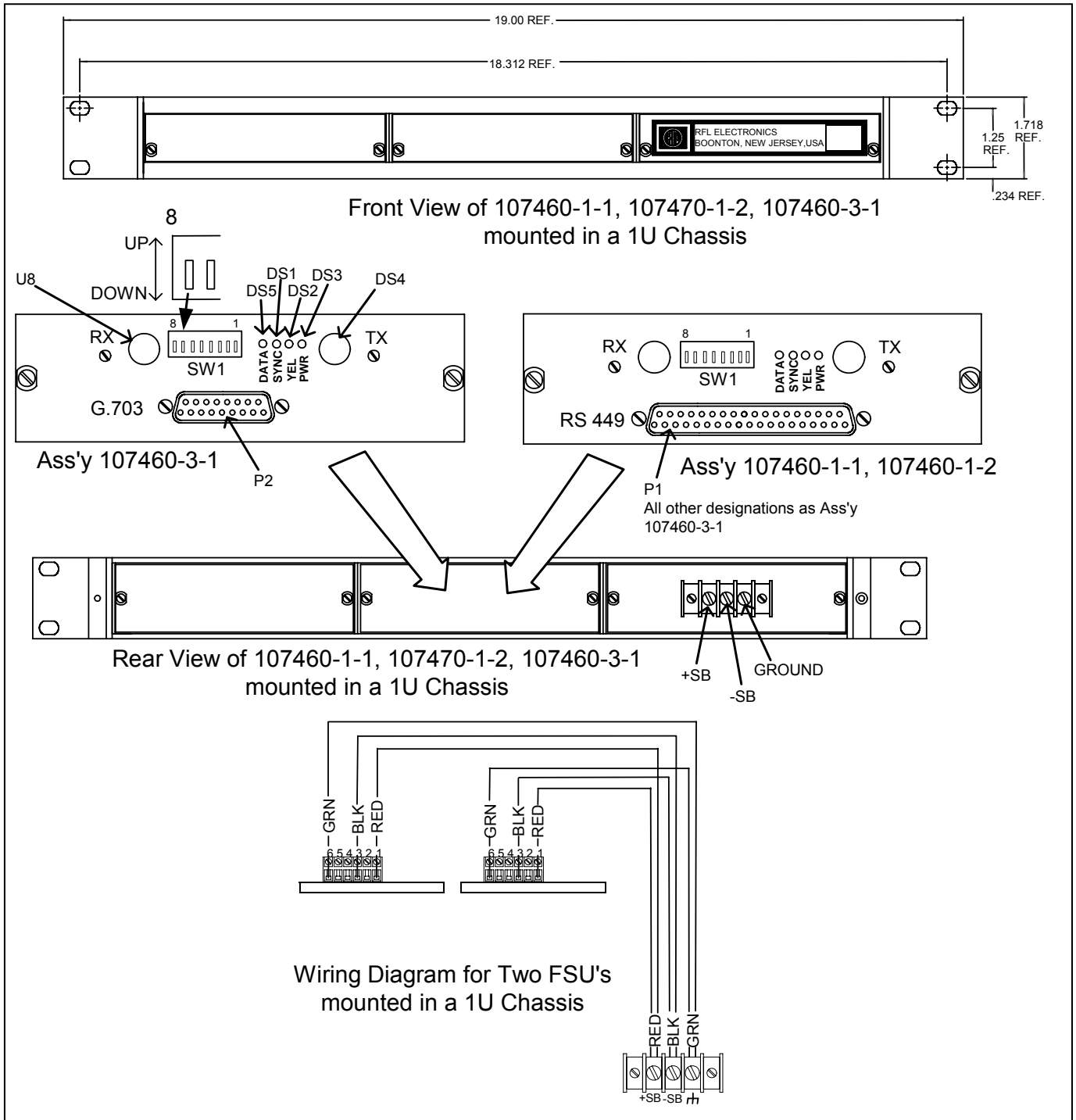
Figure 6. Fiber Service Unit, mounted in a 1U Chassis (107460-1-1, 107460-1-2, 107460-1-3)
